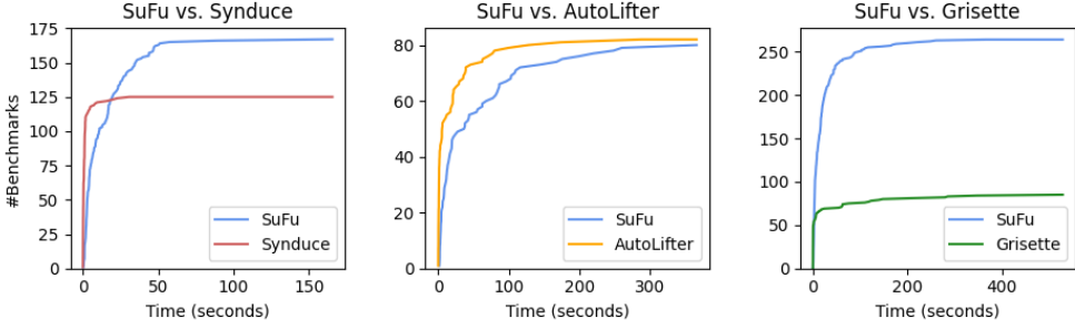
Fig. 6. Number of tasks solved by SuFu and each baseline solver over time. Comparisons with SYNDUCE and AUTOLIFTER are on their respective datasets, while the comparison with GRISLETTE is on our full dataset.
