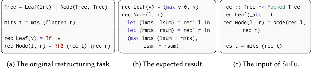
Fig. 8. An example for restructuring data structure traversals. (a) The input of the restructuring task, where mits is the reference program, and rec is the user-provided sketch. (b) The expected result of program restructuring, which introduces the sum of leaf values as an auxiliary output. (c) The corresponding input of SuFu for solving this restructuring task.
